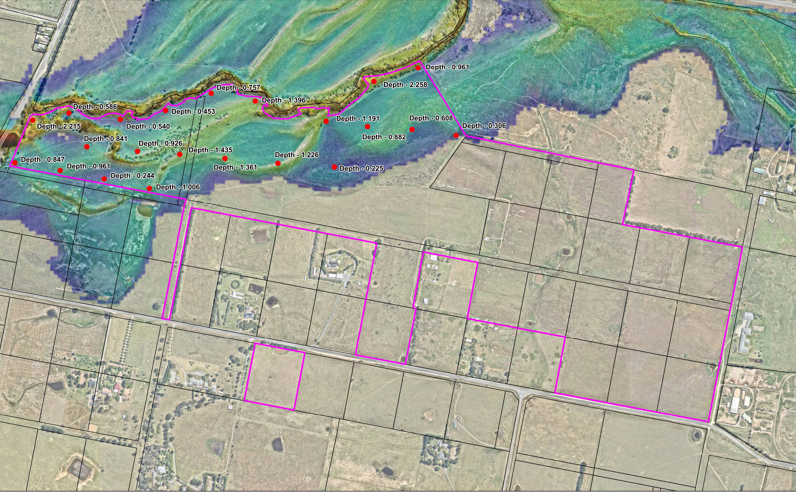
(137) Brisbane Grove Rd Subject Site- 5% Flood Depths
