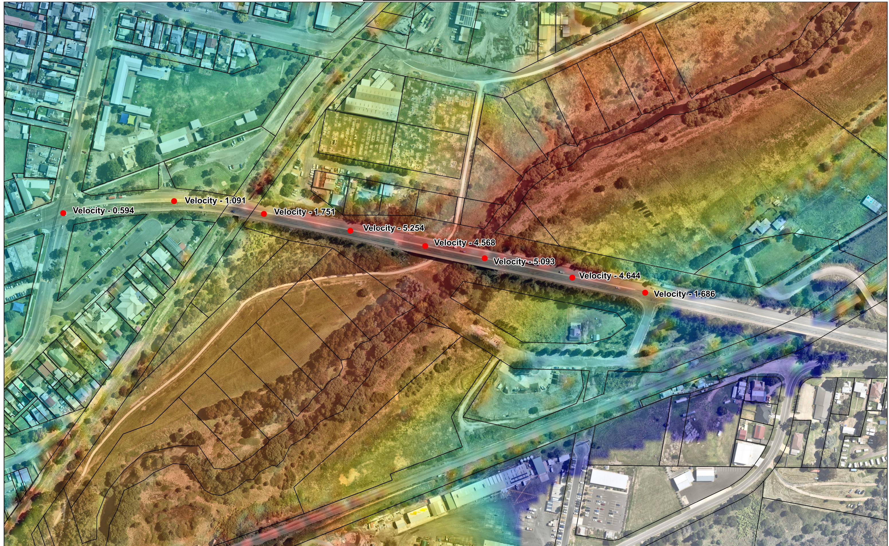
Area D- PMF Flood Velocities
