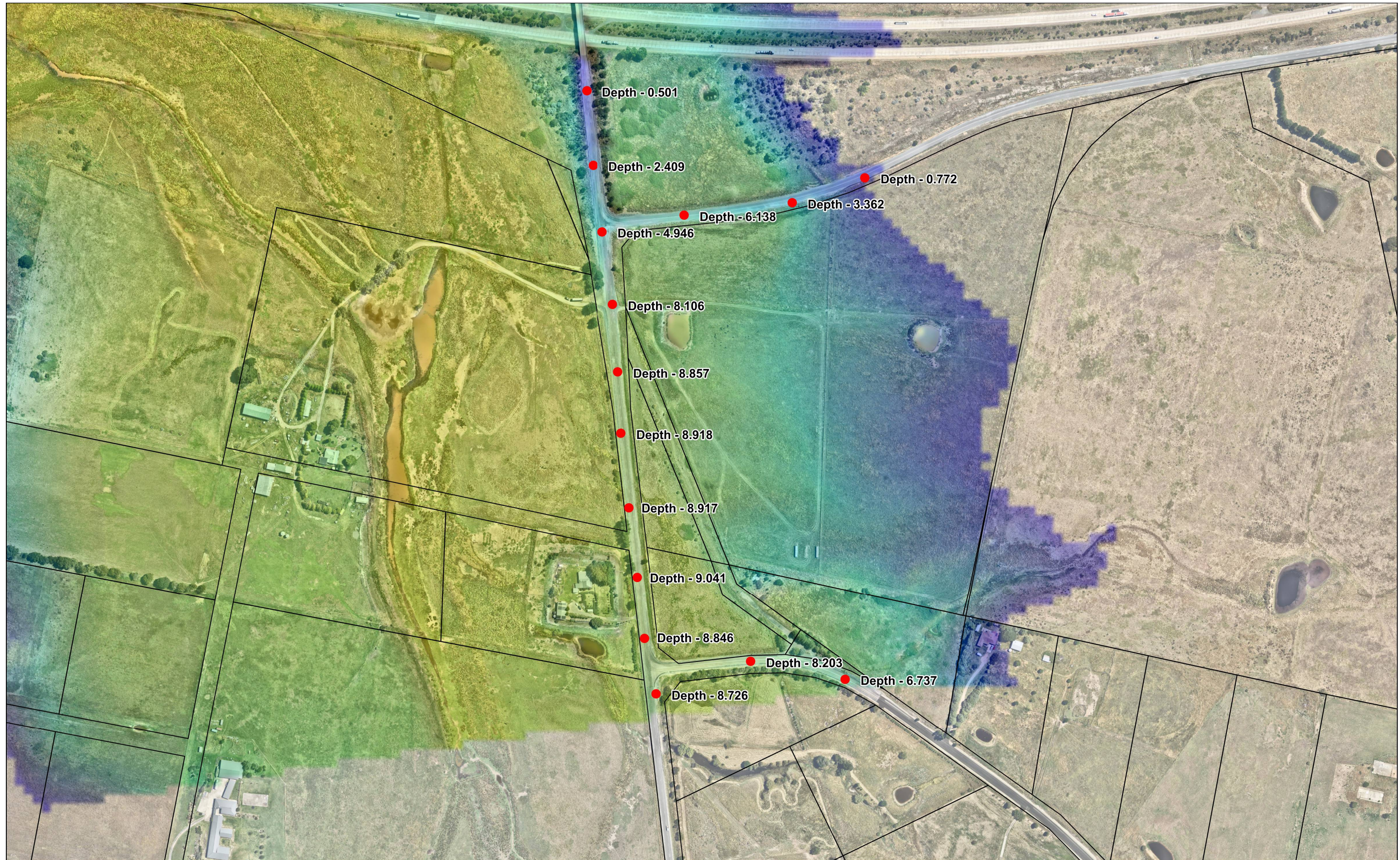
Area B- PMF Flood Depths
