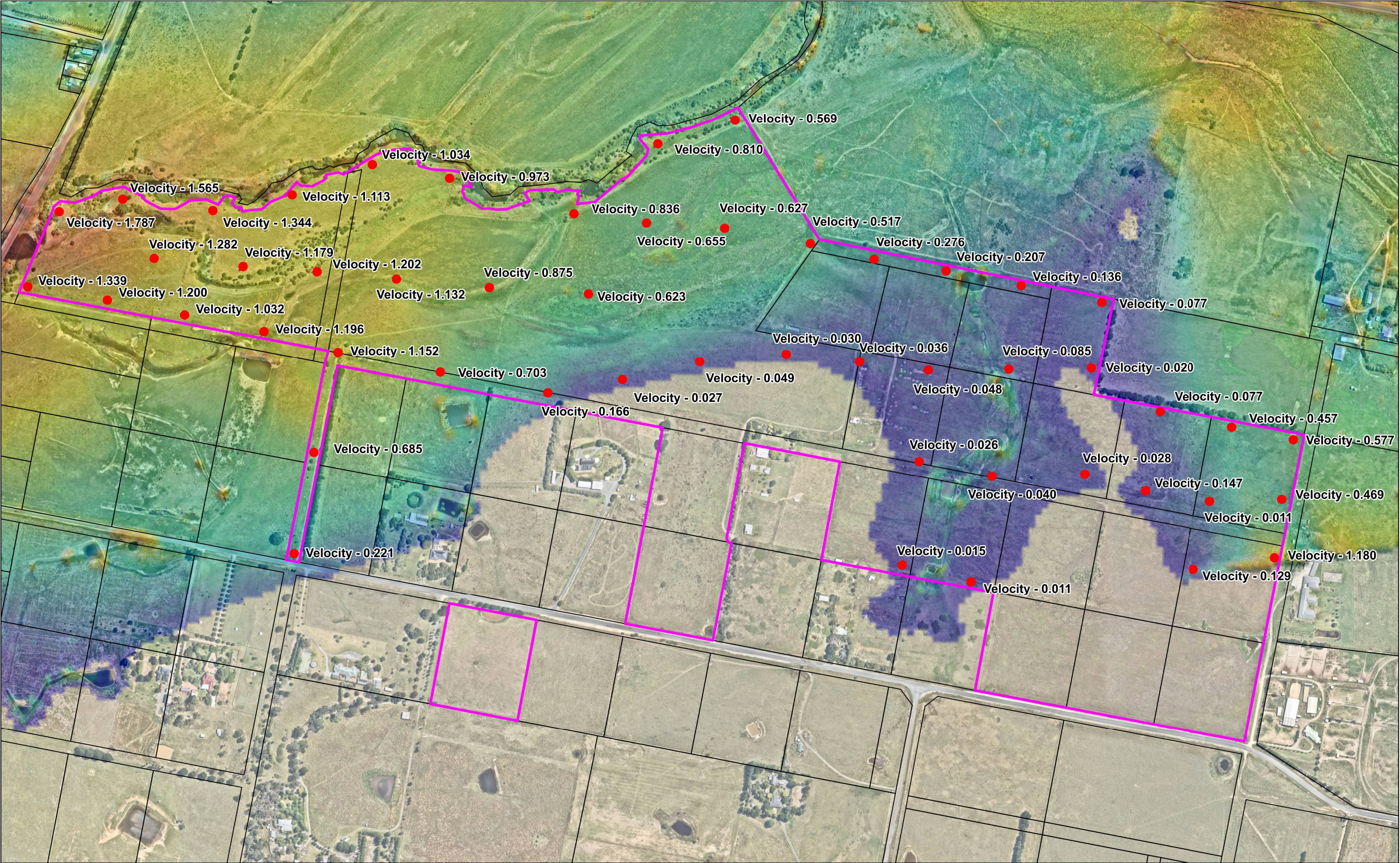
(137) Brisbane Grove Rd Subject Site- PMF Flood Velocities
