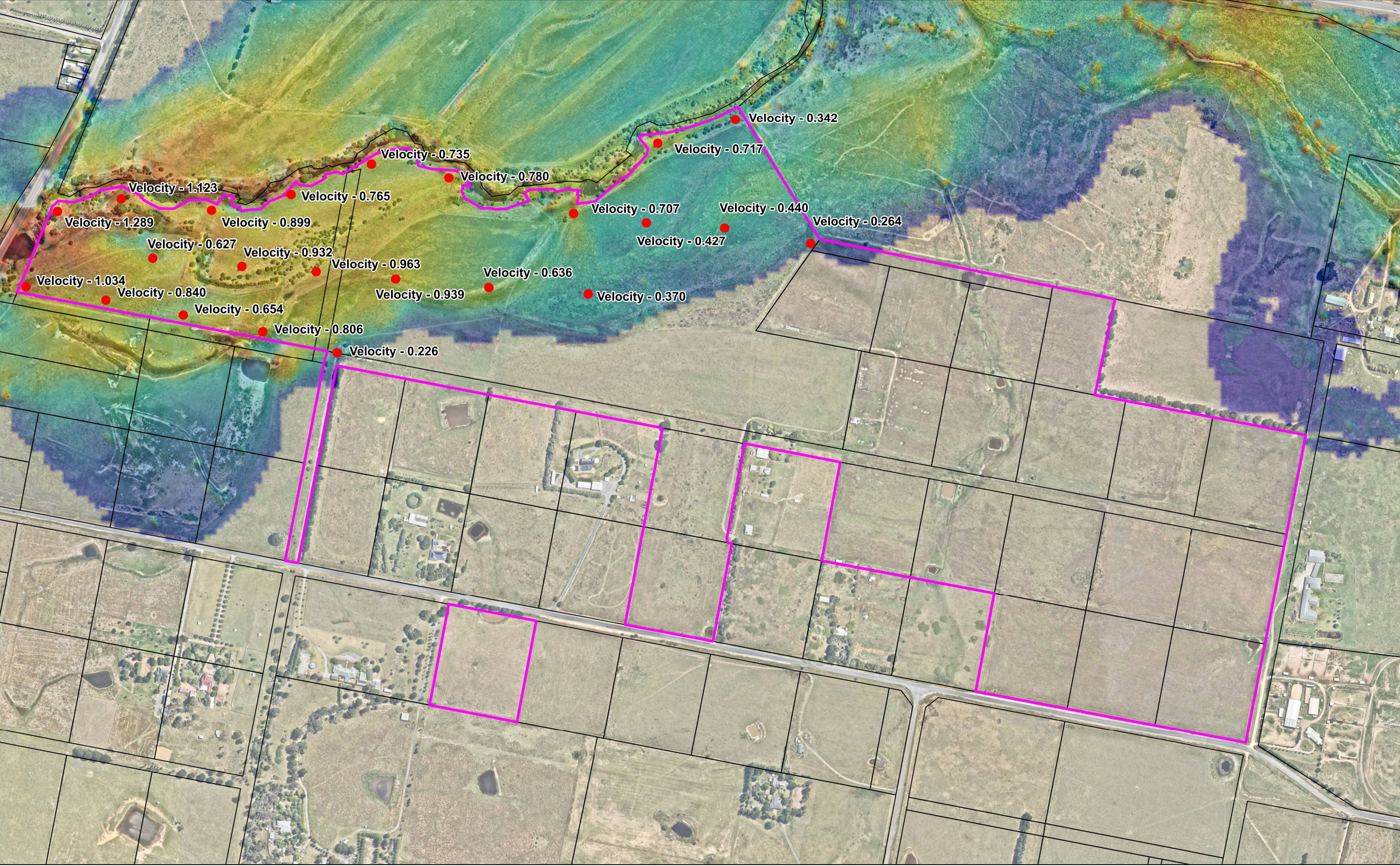
(137) Brisbane Grove Rd Subject Site- 1% Flood Velocities
