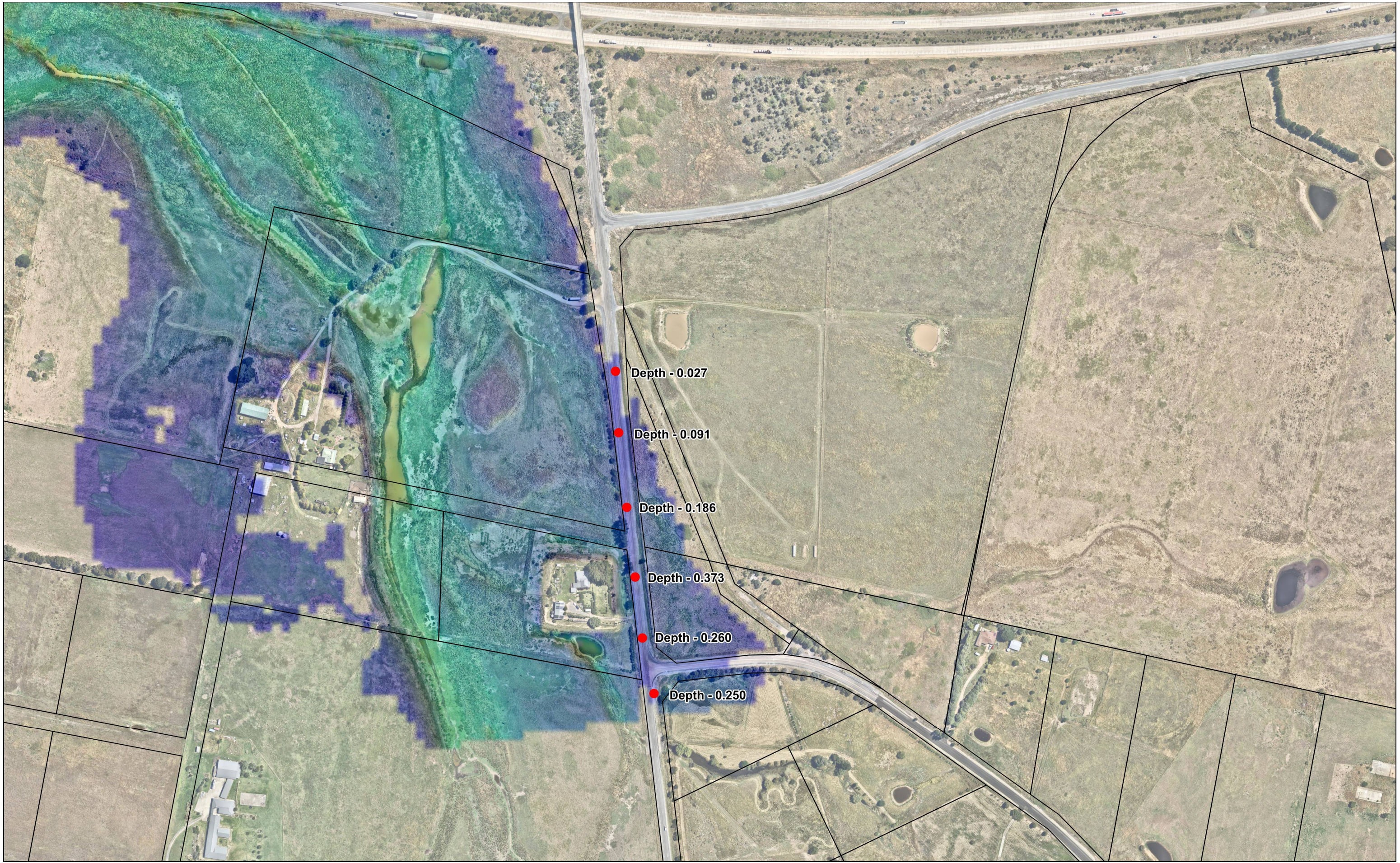
Area B- 1% Flood Depth
