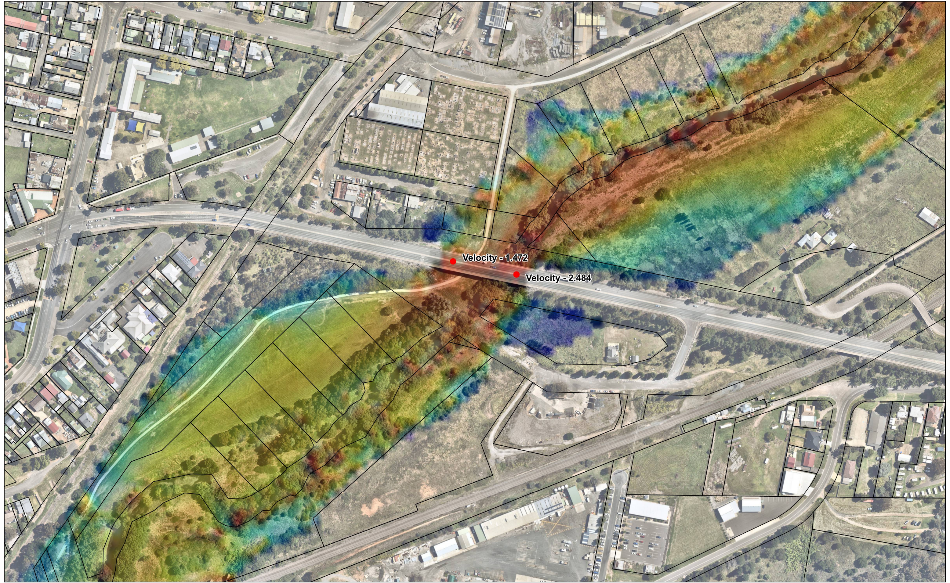
Area D- 5% Flood Velocities
