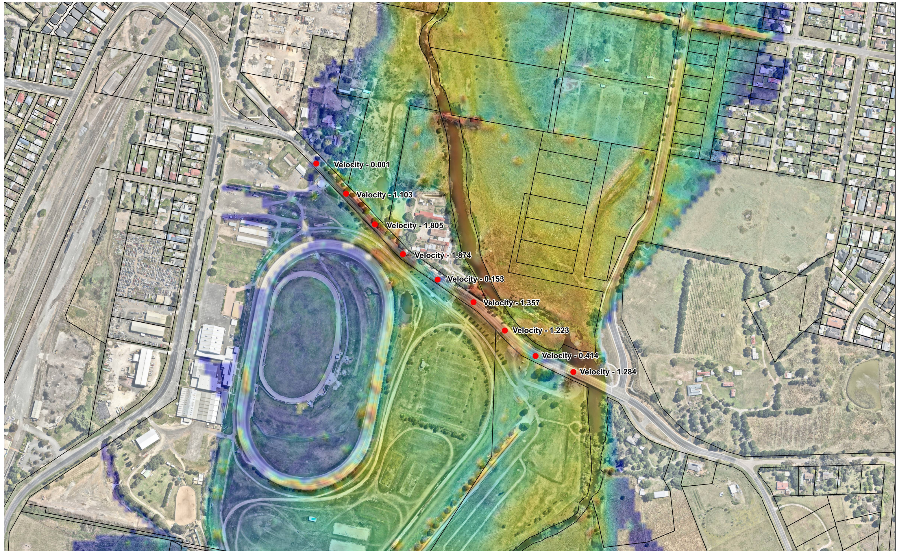
Area C- 5% Flood Velocities
