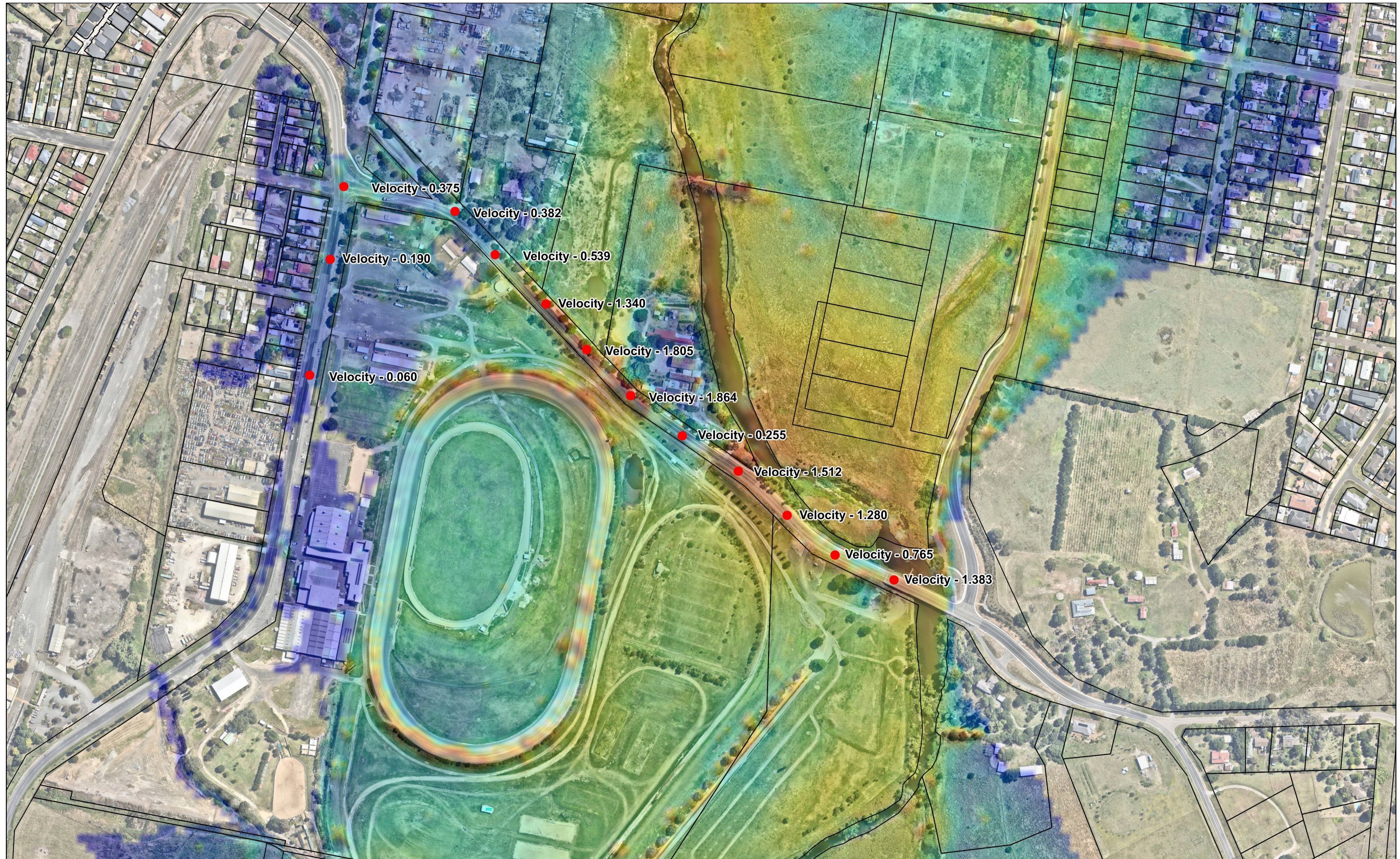
Area C- 1% Flood Velocities
