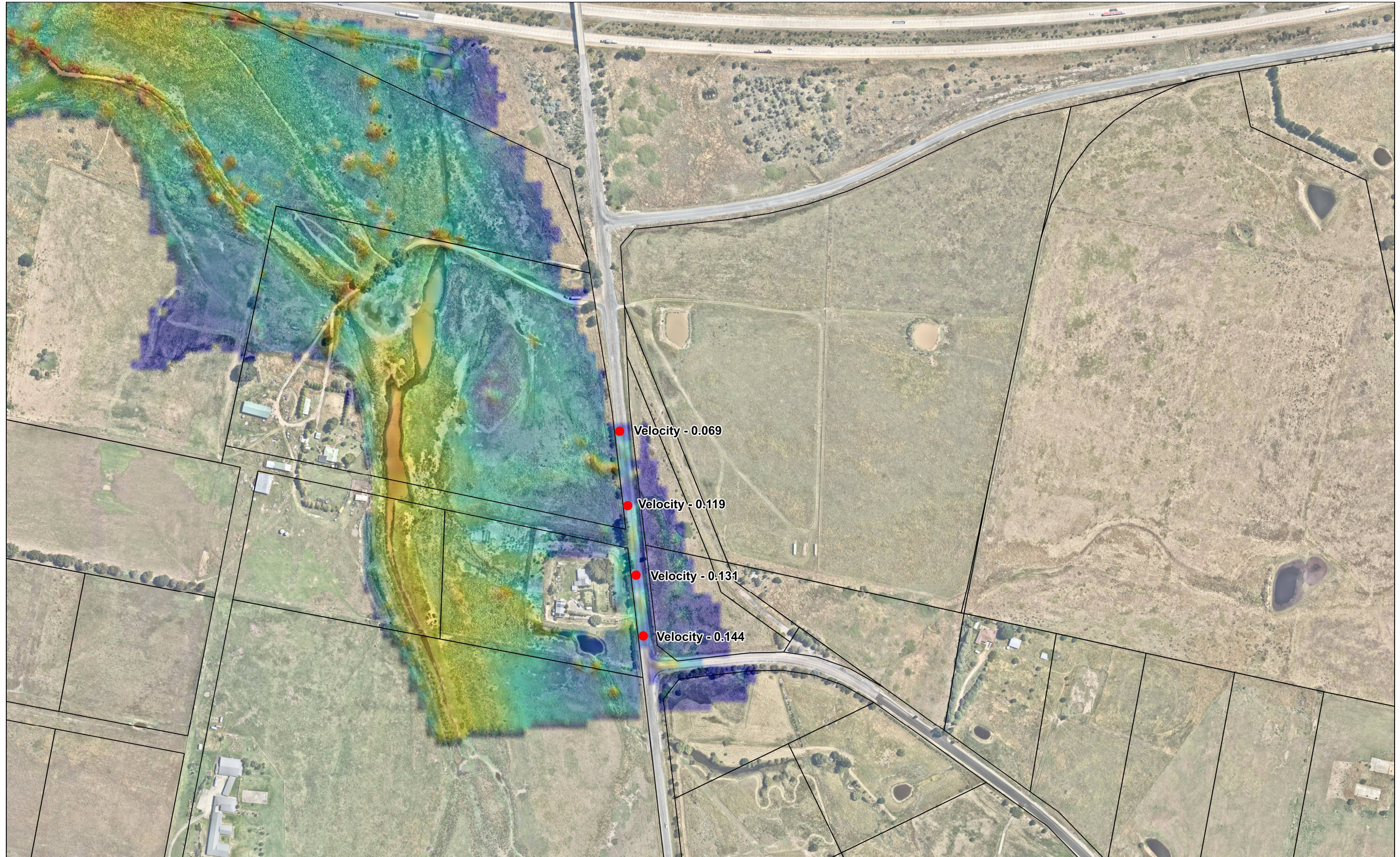
Area B- 5% Flood Velocities
