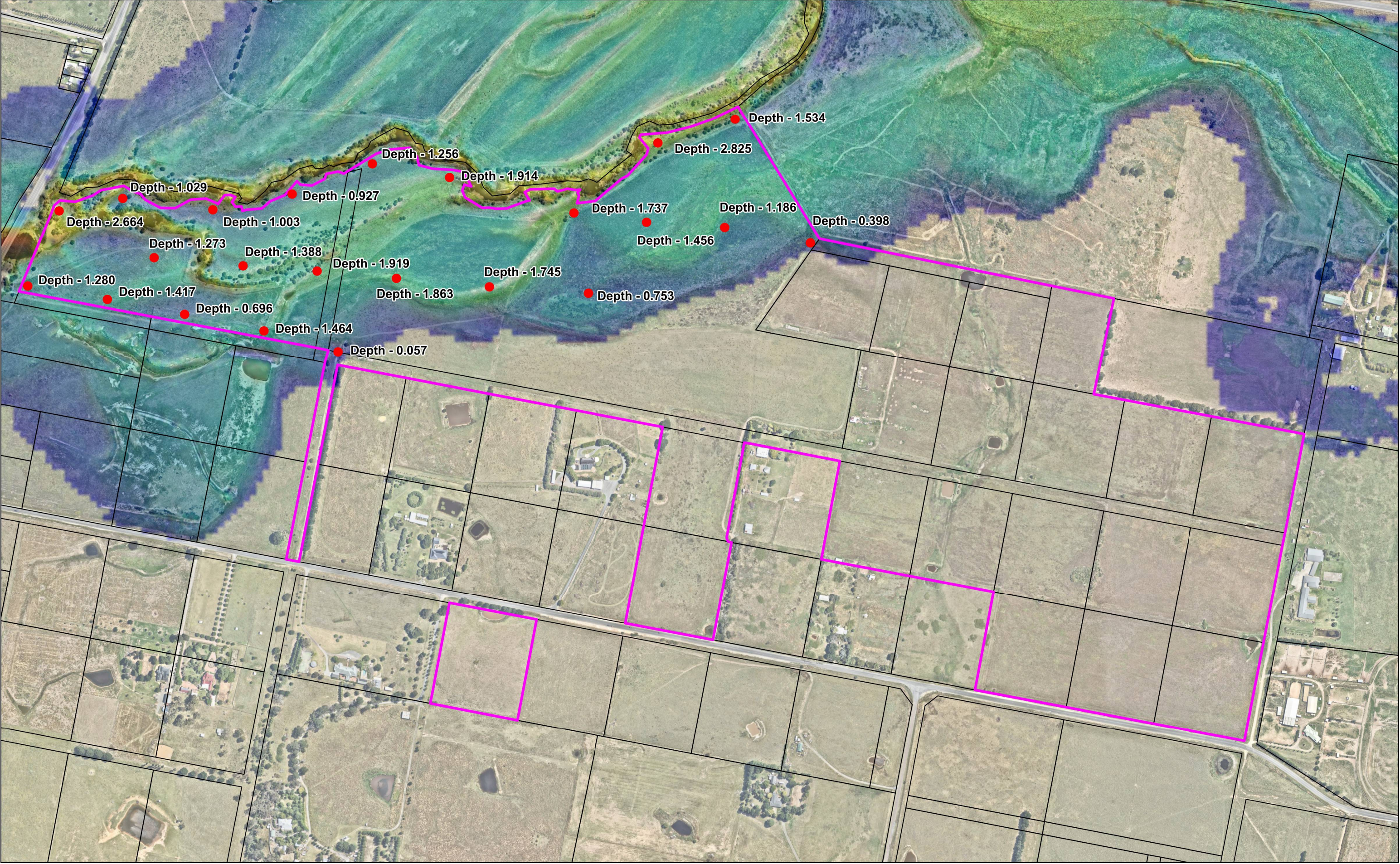
(137) Brisbane Grove Rd Subject Site- 1% Flood Depths
