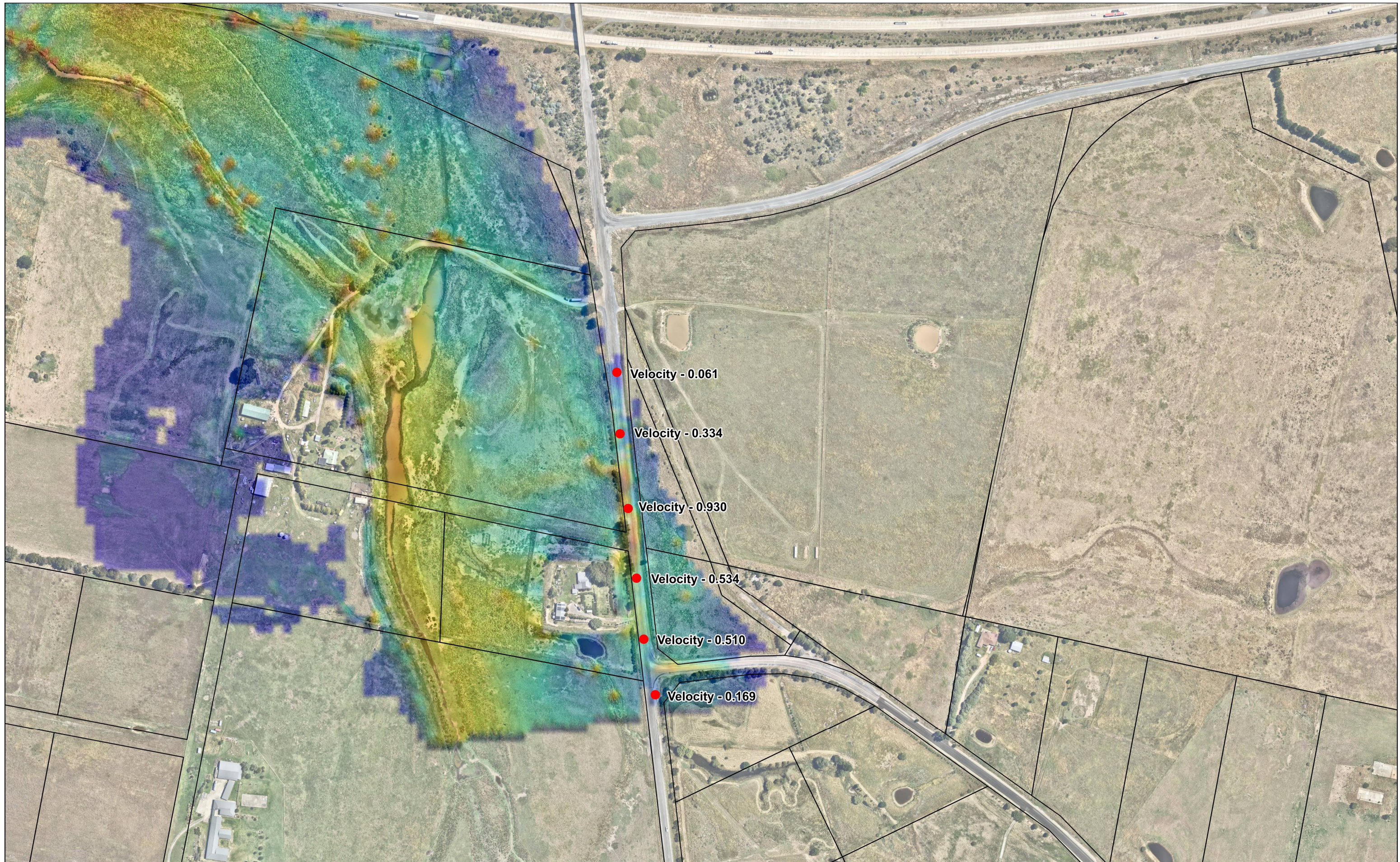
Area B- 1% Flood Velocities
