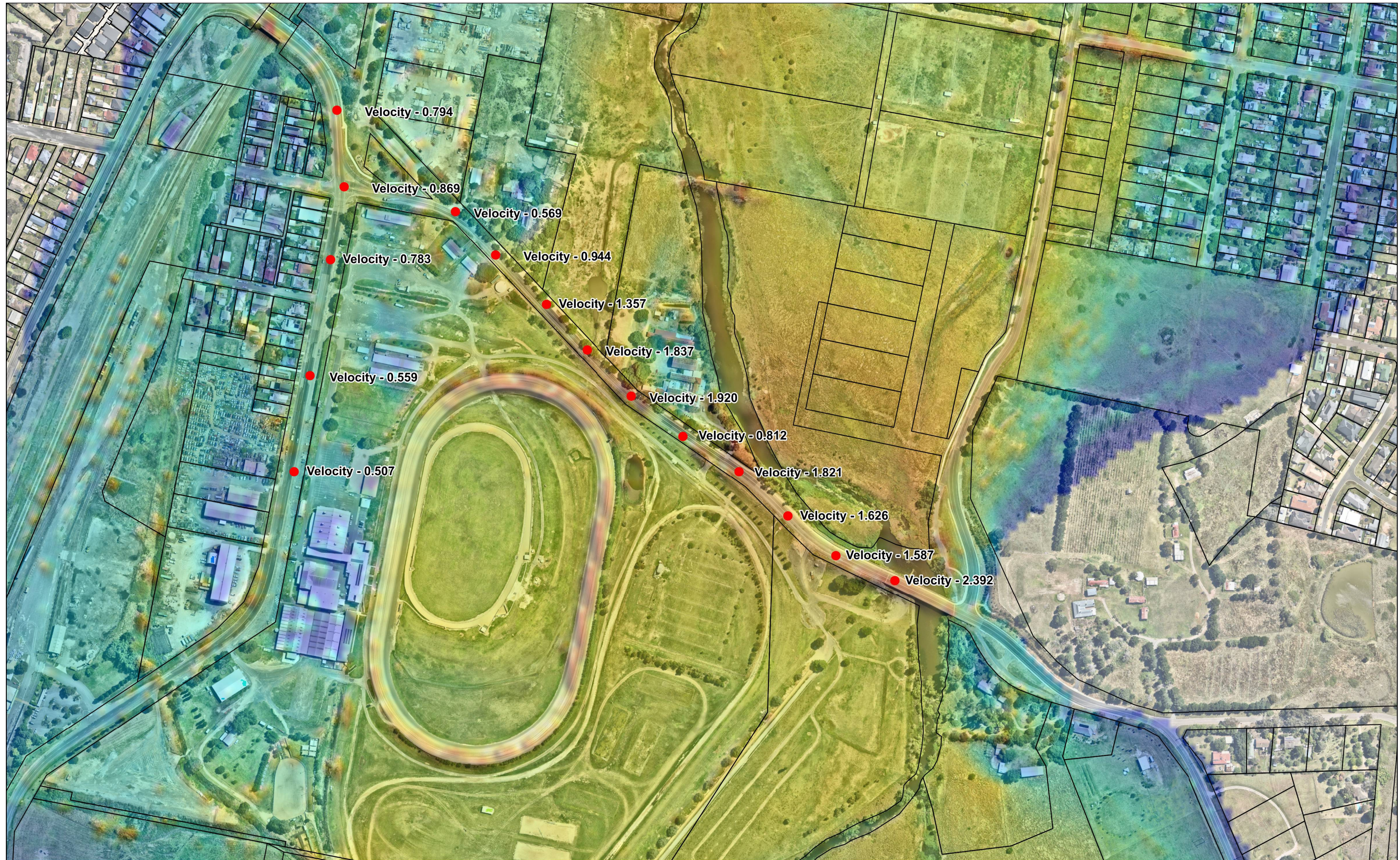
Area C- PMF Flood Velocities
