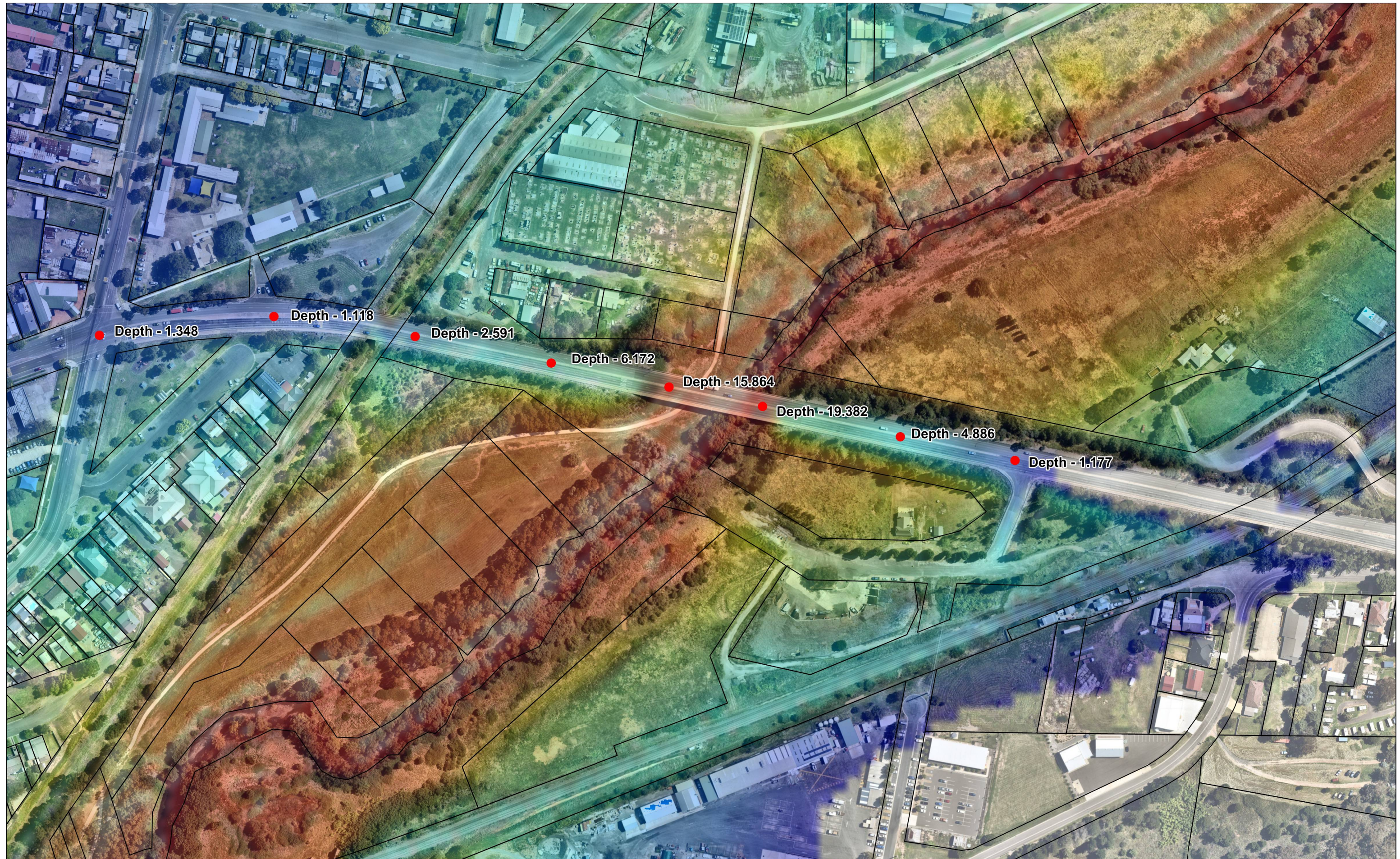
Area D- PMF Flood Depth
