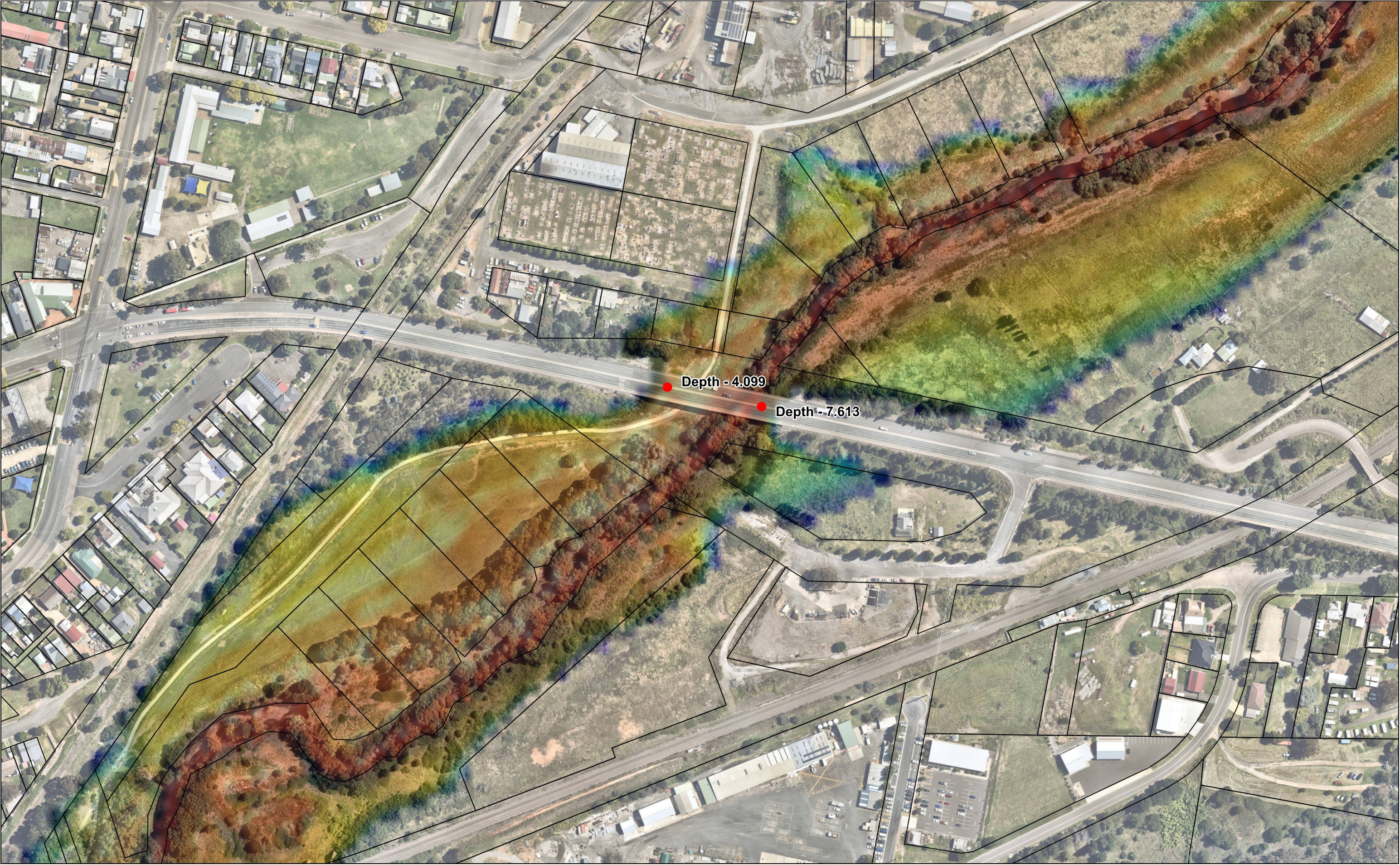
Area D- 5% Flood Depth
