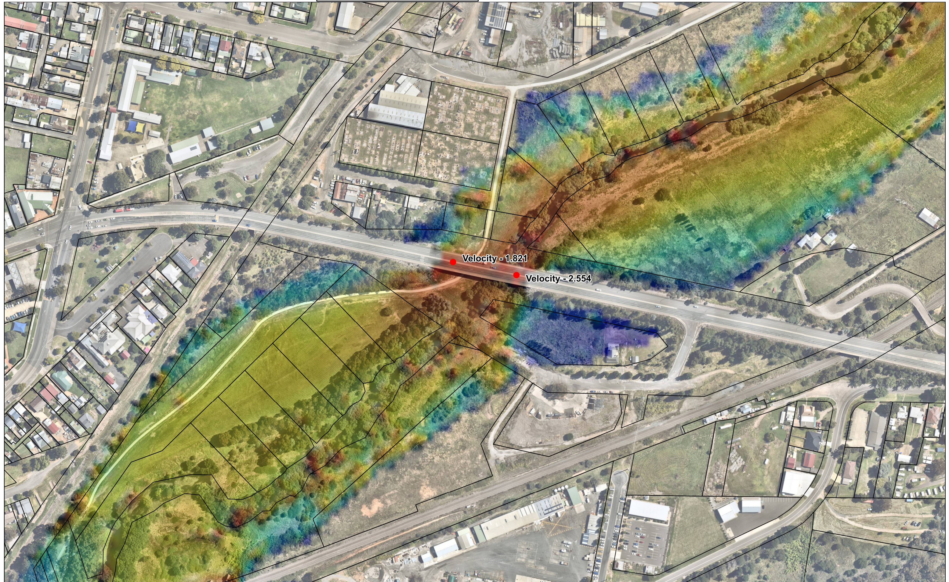
Area D- 1% Flood Velocities
