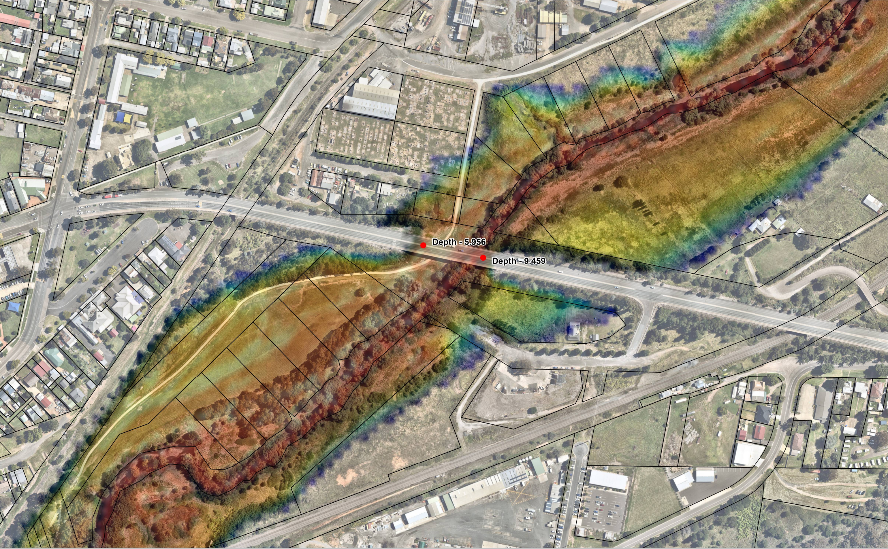
Area D- 1% Flood Depth
