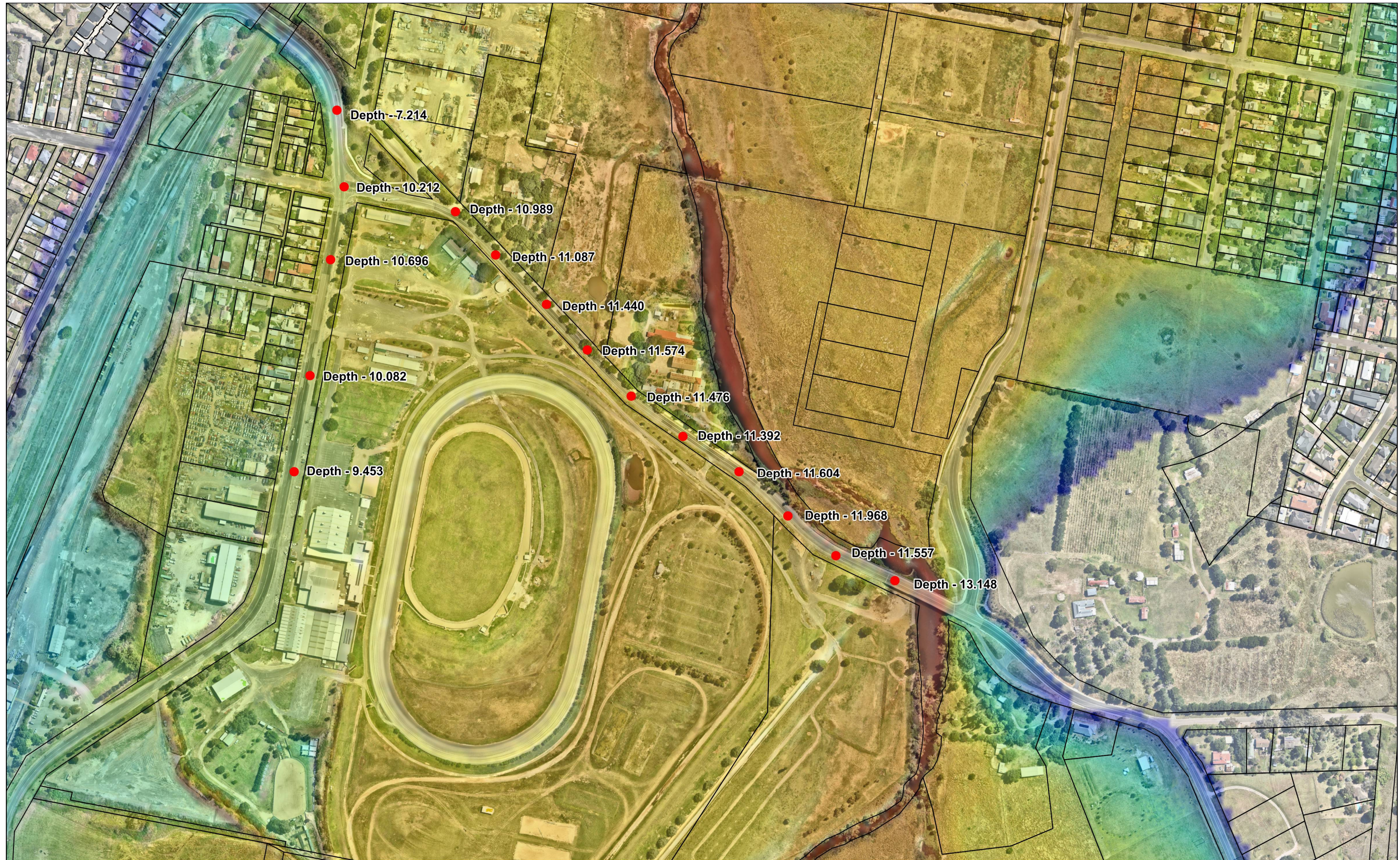
Area C- PMF Flood Depth
