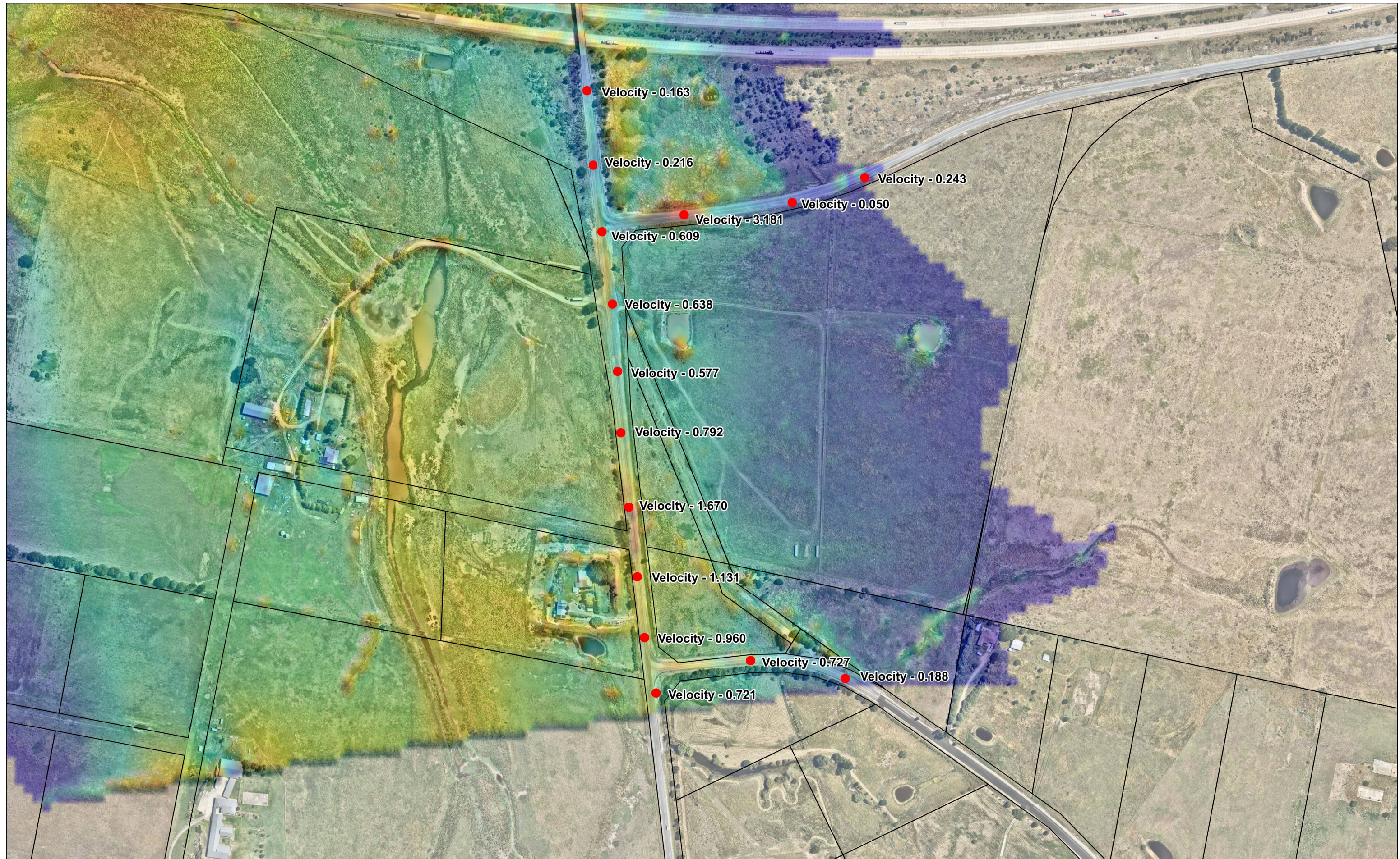
Area B- PMF Flood Velocities
